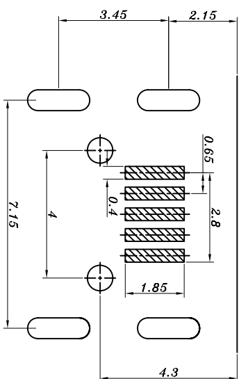
PCB LAYOUT
