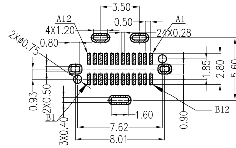
RECOMMENDED PCB LAYOUT (t=0.80±0.05) COMPONENT SIDE (GENERAL TOLERANCE: ±0.05)
