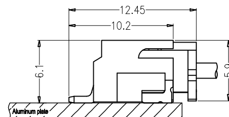
ASSEMBLY LAYOUT
