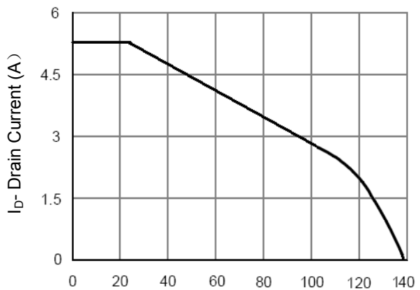
Figure 4 Drain Current
