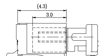
MATED CONDITION
