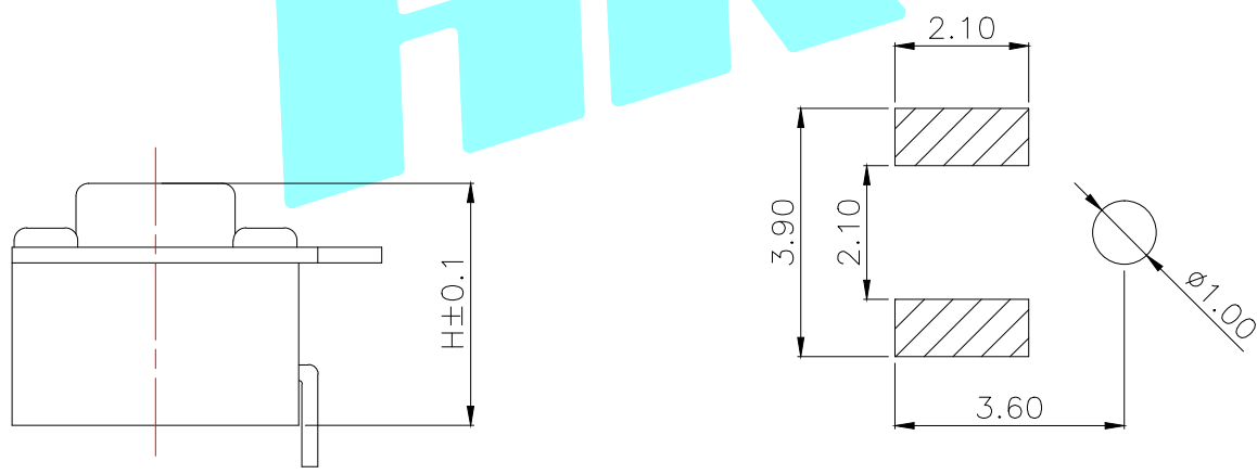
PCB Layout
