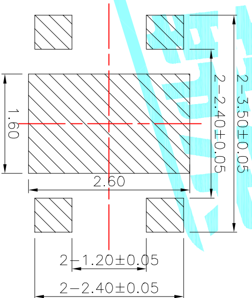
PCB Layout (Pattern Side)
