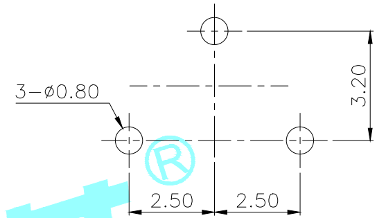
HOLE LAYOUT
