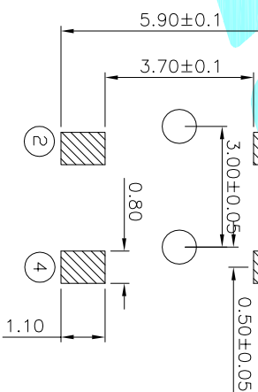
PCB LAND DIMENSION
