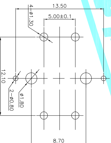
PCBLayout(pattern Side)
