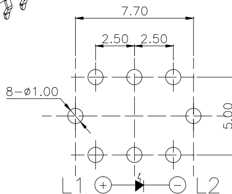
PCBLayout(Pattern Side)
