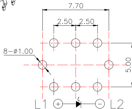
PCBLayout(Pattern Side)
