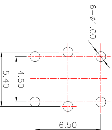
PCBLayout(Pattern Side)
