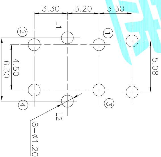
PCBLayout(Pattern Side)
