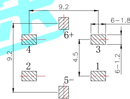
PCBLayout(Top view)
