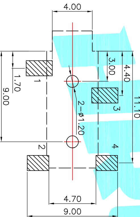
P.C.B LAYOUT(copper-side view)
