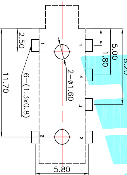
P.C.B Layout (copper-sided view)
