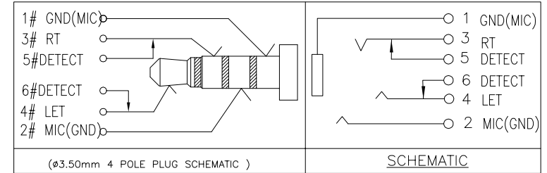
(φ3.50mm 4 POLE PLUG SCHEMATIC )
