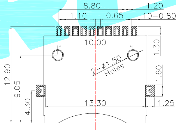
PCB Layout(TOP Side)
