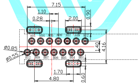
RECOMMENDED P.C.B. LAYOUT <T:1.00mm> TOLERANCE UNSPECIFIED ±0.05mm
