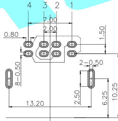
RECOMMENDED P.C.B. LAYOUT TOLERANCE UNSPECIFIED ±0.1mm
