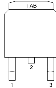
TO-252-3L
