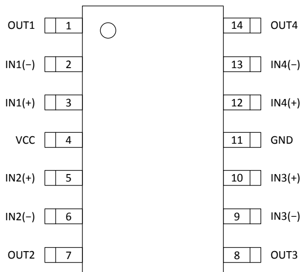
SOP-14
