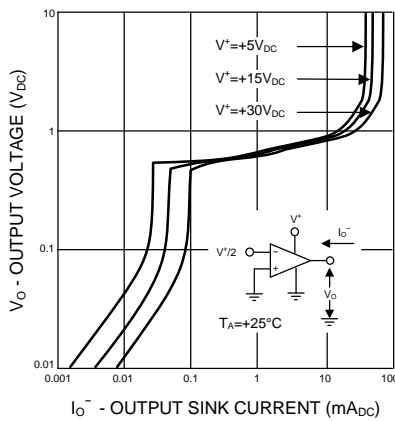
OUTPUT CHARACTERISTICS CURRENT SINKING
