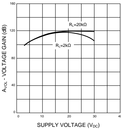
VOLTAGE GAIN
