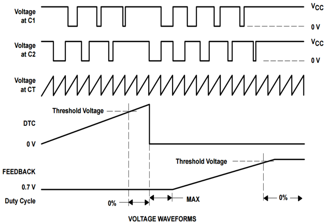
FIGURE 1. OPERATIONAL TEST CIRCUIT AND WAVEFORMS
