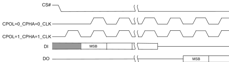
Figure 6.1 SPI Modes
