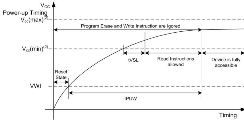
Figure 8.1 Power-up Timing
