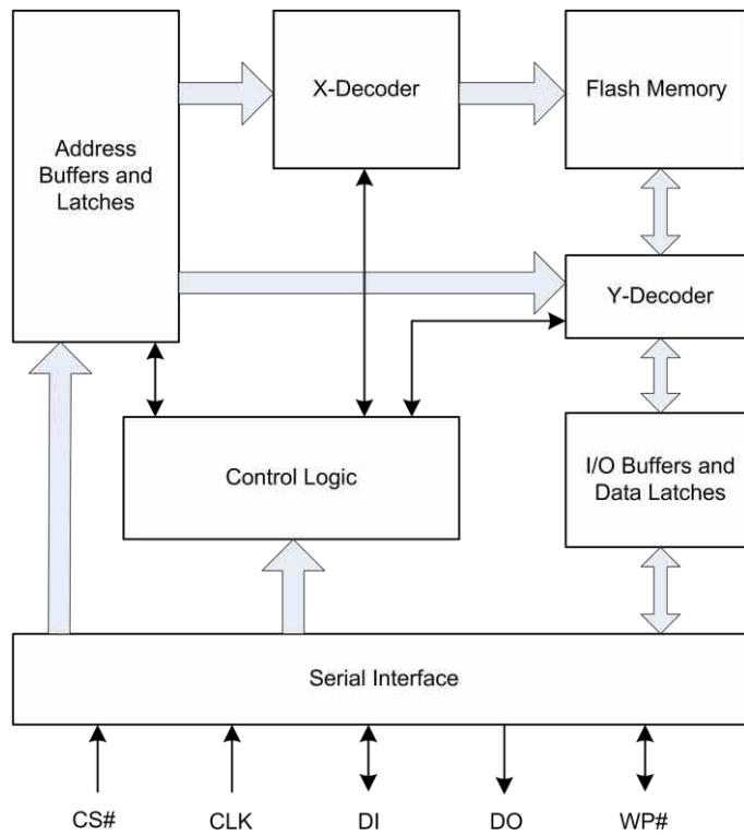
Figure 2.1 Block Diagram
