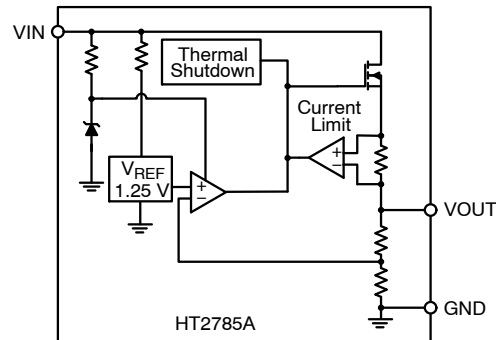
Figure 2. Simplified Internal Block Diagram
