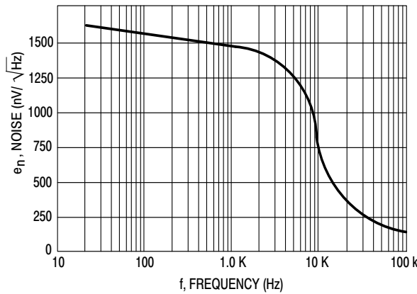
Figure 12. Noise Voltage
