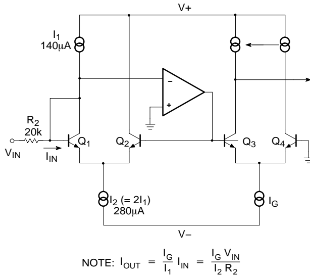
Figure 12. Simplified ΔG Cell Schematic
