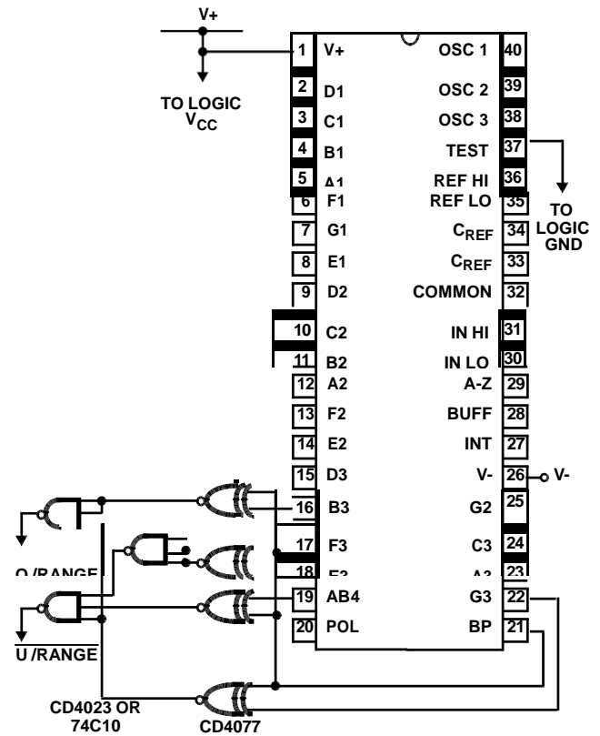
FIGURE 11. CIRCUIT FOR DEVELOPING UNDERANGE AND OVERRANGE SIGNAL FROM HT7126A OUTPUTS
