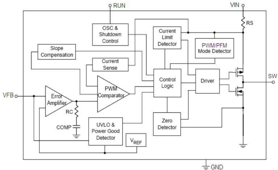
Figure 2. HT8008A Block Diagram
