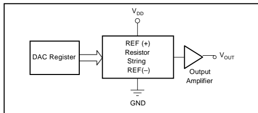
FIGURE 1. HT8312A Architecture.
