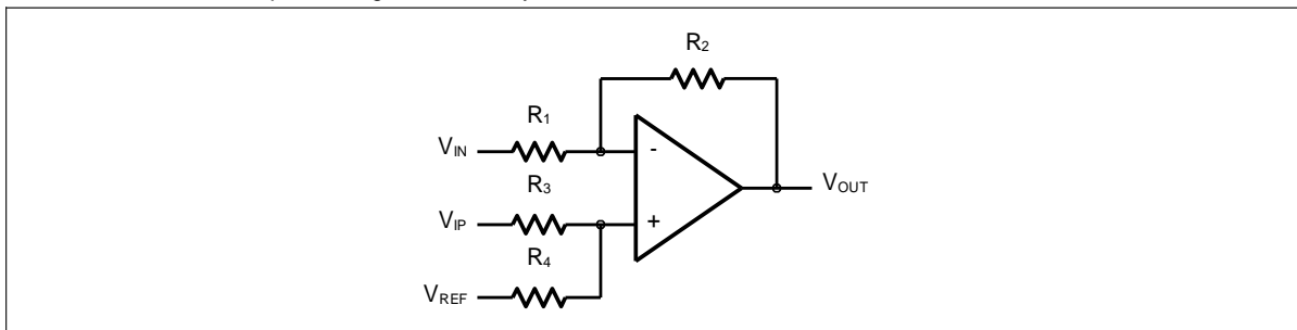
Figure 4. Differential Amplifier
