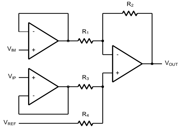
Figure 6. Instrument Amplifier
