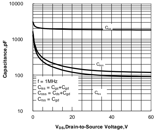
Figure 12. Capacitance Characteristics
