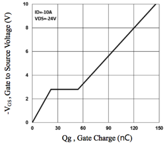
Fig.4 Gate-Charge Waveform
