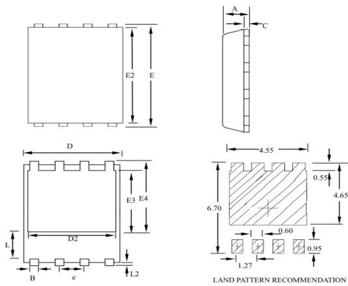
PRPAK5*6 Outline
