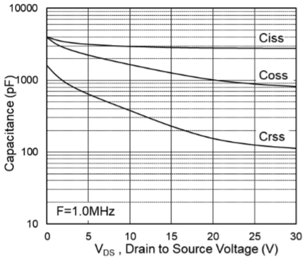
Fig.7 Capacitance
