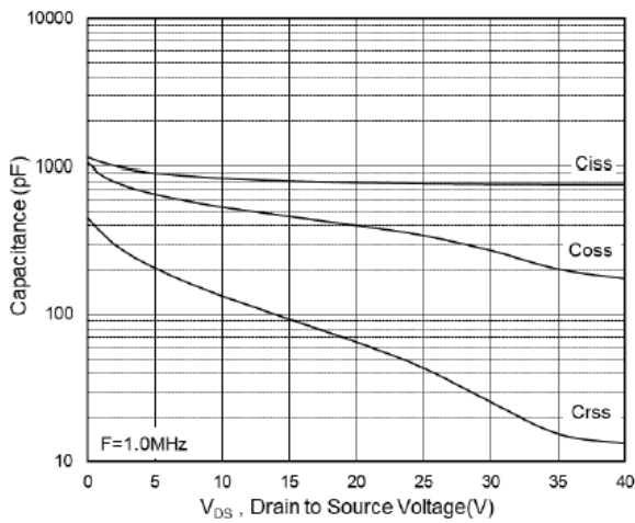
Fig.7 Capacitance
