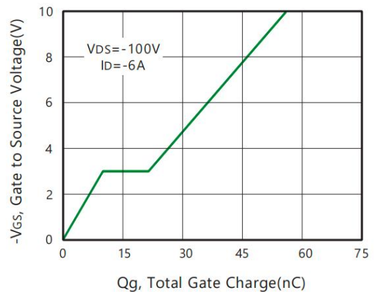
Figure 6. Gate Charge
