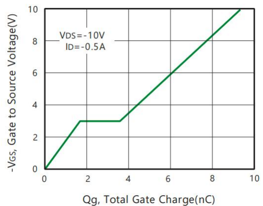
Figure 6. Gate Charge
