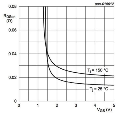
Fig.2 On-Resistance vs. Gate-Source
