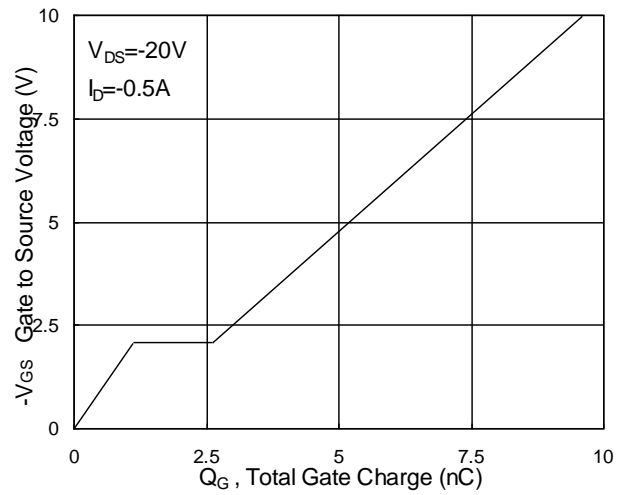
Fig.2 Gate-Charge Characteristics
