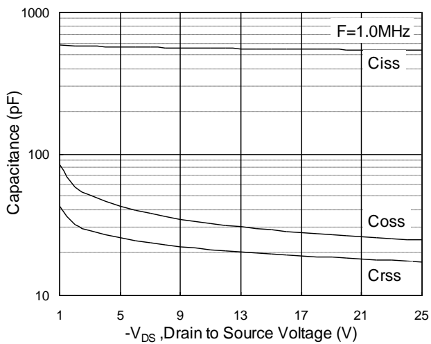
Fig.5 Capacitance
