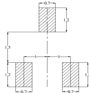
(For reference only) Land Pattern
