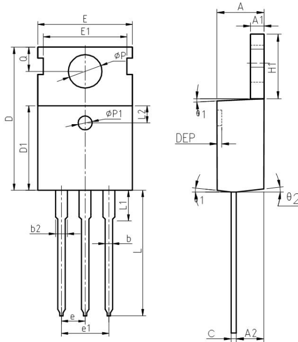
COMMON DIMENSIONS
