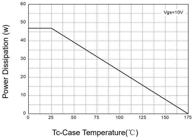
Figure 1: Power Dissipation
