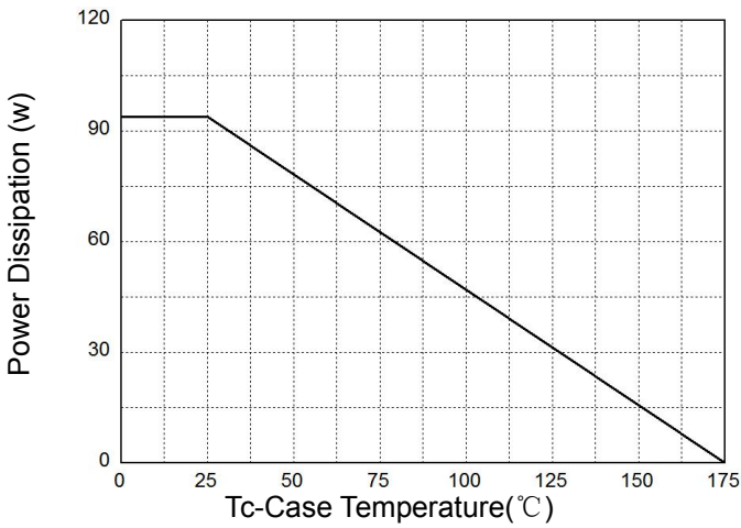
Figure 1: Power Dissipation
