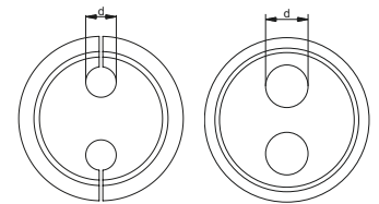
Slit version
