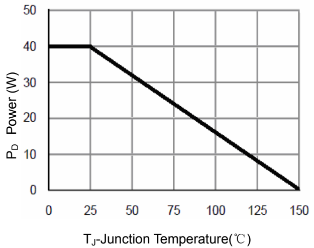
Figure 9 Power Dissipation
