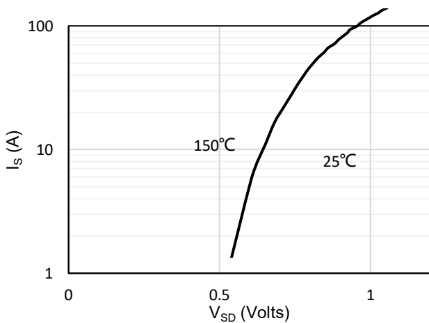
Figure 5: Body-Diode Characteristics
