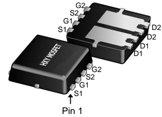
DFN3X3-8L
