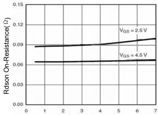
ID- Drain Current (A) Figure 6 Drain-Source On-Resistance
